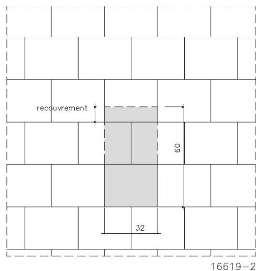
Fig. 6: Format 60/32
