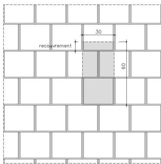
Fig. 9: Format 60/30
